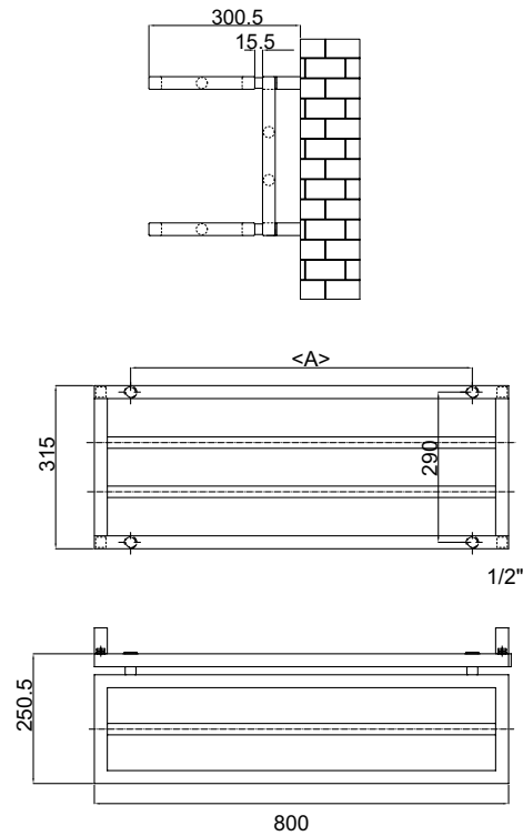
SMART U nipped/hiplat ( for chrome plated/ pentru cromat)
